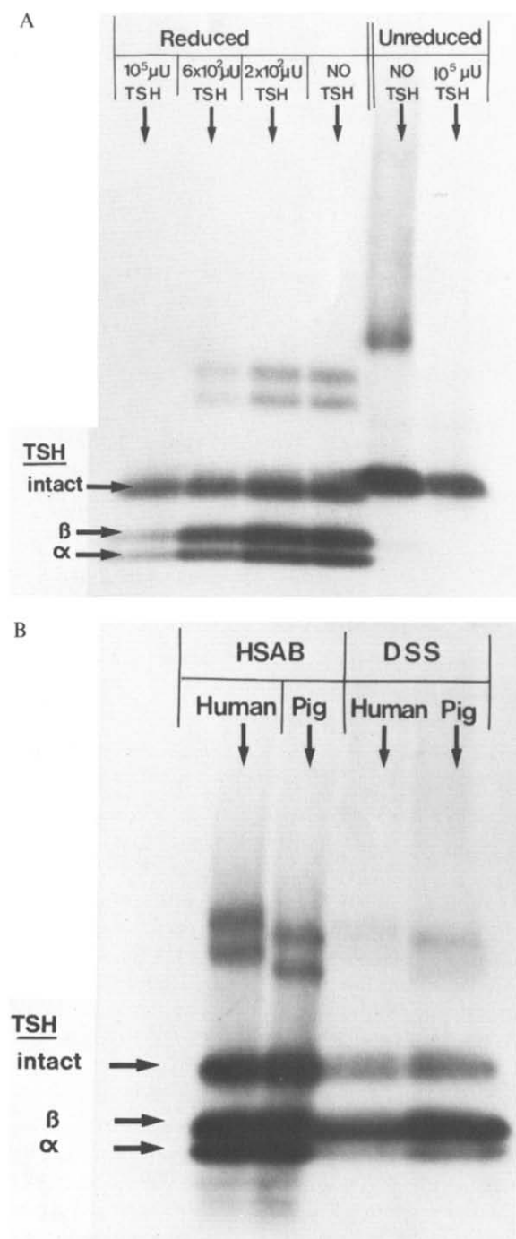
Fig.2. (A) A comparison of reduced and unreduced crosslinked complexes of ^{125}\text{I} -labelled HSAB-TSH and porcine TSH receptors. The amounts of unlabelled TSH included in the incubations are shown at the top of the autoradiograph. (B) A comparison of reduced HSAB or DSS crosslinked complexes obtained using porcine and human TSH receptors. The data shown are typical of several separate experiments (see table 1).
